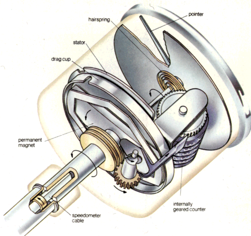
Figure 1. Cut away view of a typical speedometer.
