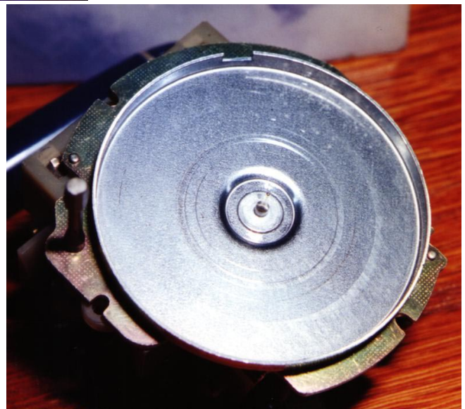
Figure 4. Now the odometer wheel frame has been removed from the magnet wheel frame. This is a view of the underside of the odometer wheel frame with the attached drag cup. In the center of the drag cup is
